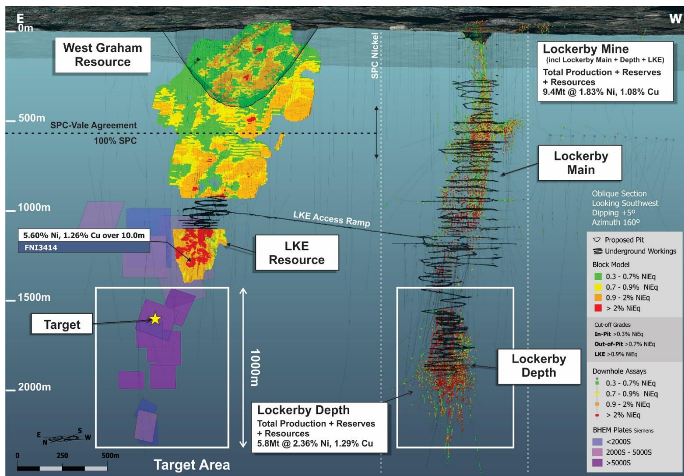
Figure 1: Long section of the Lockerby East Property and the adjacent past producing Lockerby Mine. On the east side (left) the figure shows the mineral resource and geophysical conductors associated with the West Graham – LKE mineralized system extending from surface to a depth of 2,000 metres. The current target area is shown in the white box, and the planned drill hole intersection is marked by the yellow star. To the east is the past producing Lockerby Mine system that includes the Lockerby main and depth zones. Shown in the figure are the historical drill hole assays from the Lockerby Mine used to approximate the location of the Lockerby Mine mineralized zone. The diagram does not distinguish between areas of past production, reserves or resources.
