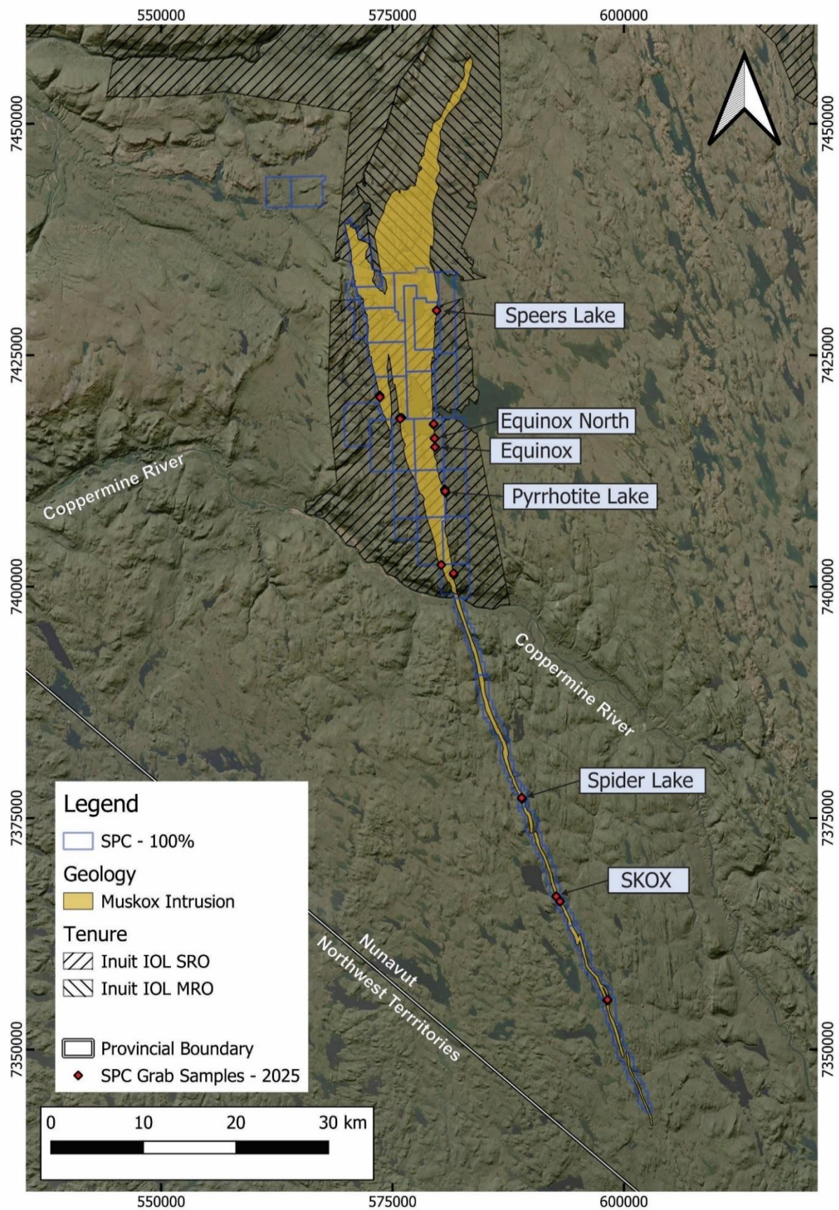
Figure 1: Regional satellite view of the Muskox Project showing the location of samples and selected Target Areas from the 2025 Field Program.
