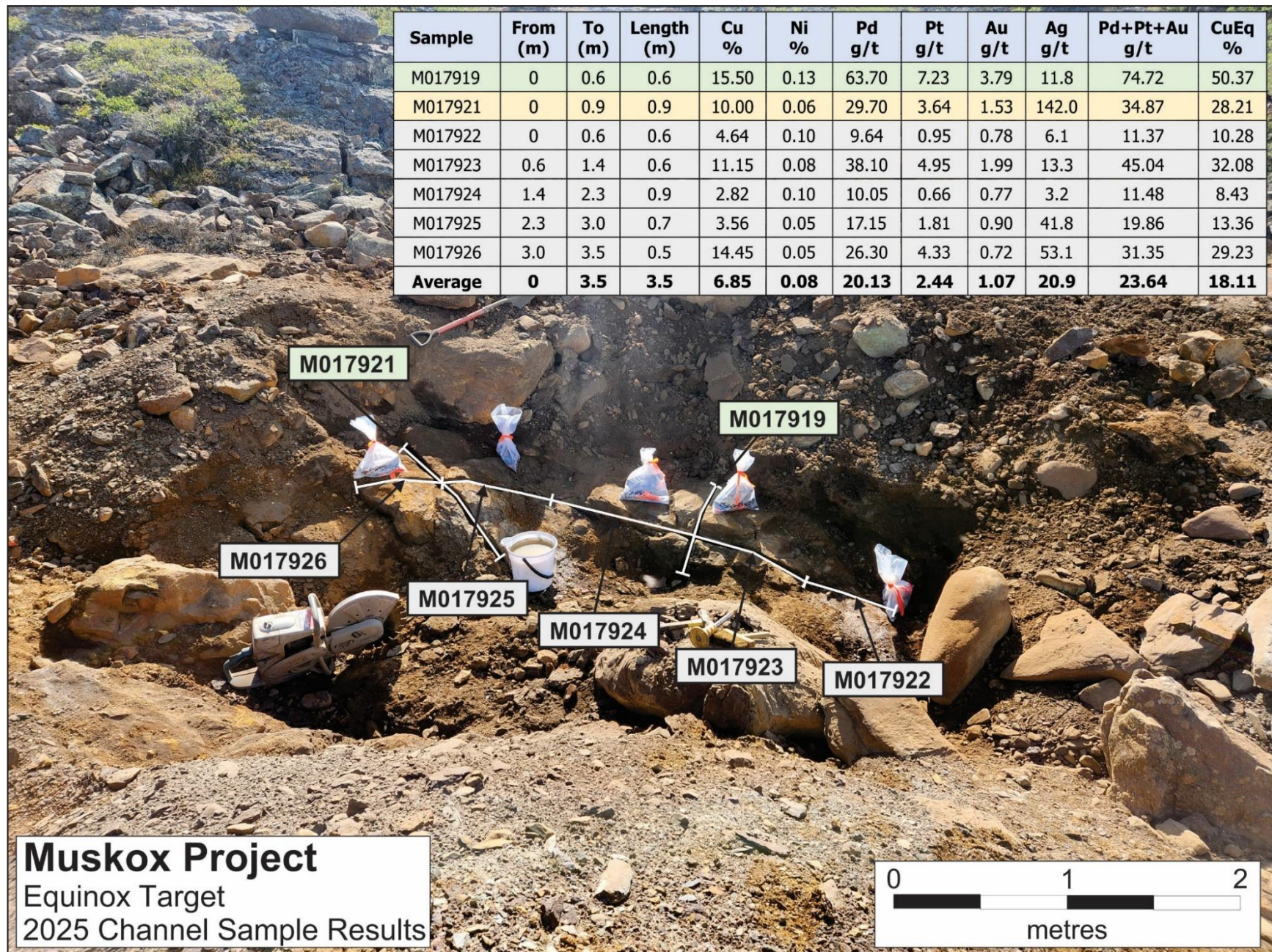
Figure 4: Photo of the historical Equinox Target showing the location of the Channel Samples completed during the 2025 Field Program.
