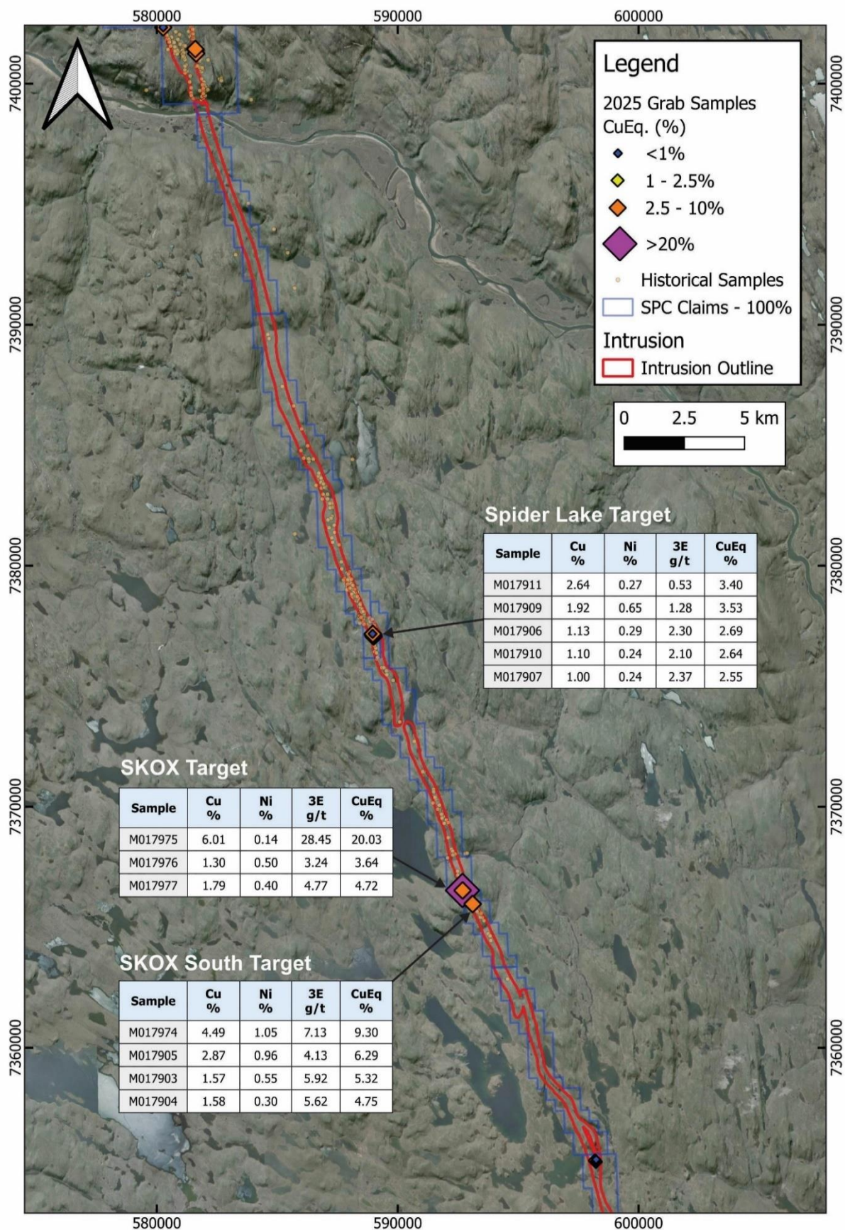
Figure 3: Regional satellite view of the Muskox Project (Feeder Dyke) showing the location of samples and selected assays from the 2025 Field Program.
