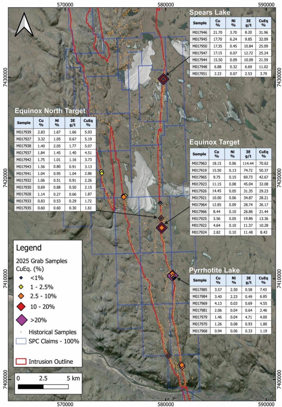
Figure 2: Regional satellite view of the Muskox Project (Main Muskox Intrusion) showing the location of samples and selected assays from the 2025 Field Program.
