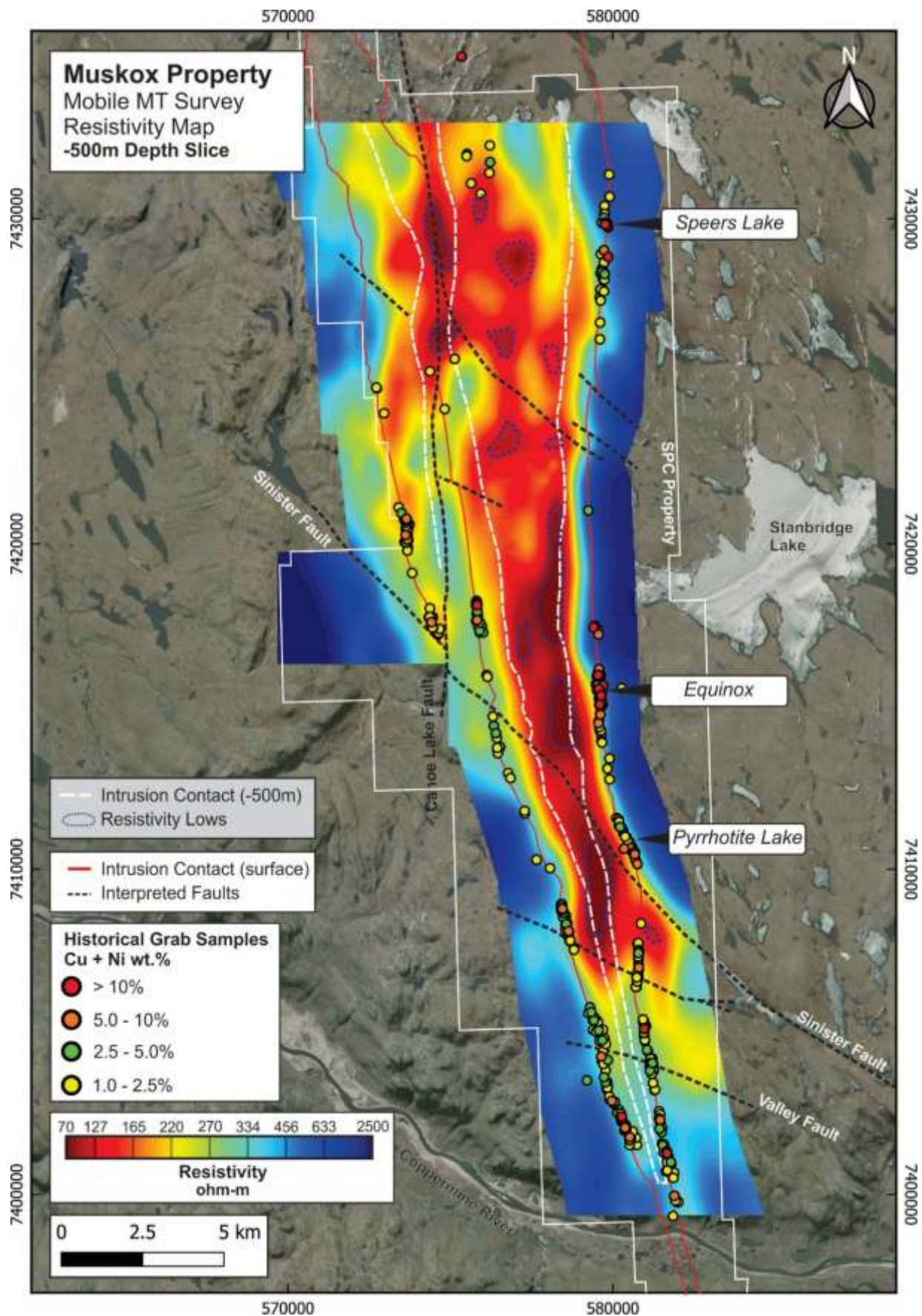
Figure 2: Muskox MMT Imagery (Resistivity Map) -500 metre depth slice overlaying historical surface grab samples, major structures, interpreted Muskox geological contact at -500 metres, modeled zones of low resistivity and the Company's current property position. Grab samples are selective in nature and are not representative of the overall mineralized system.
