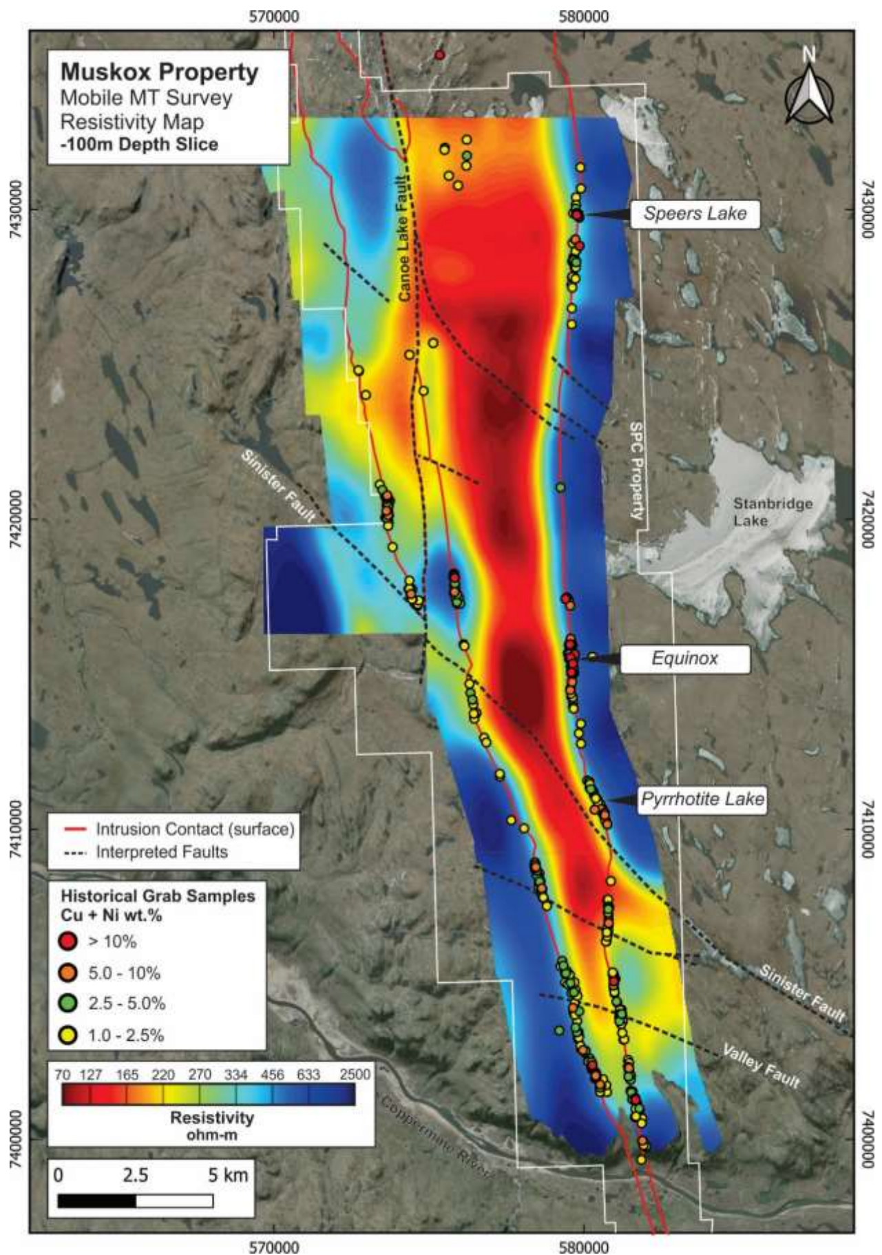
Figure 1: Muskox MMT Imagery (Resistivity Map) -100 metre depth slice overlaying historical surface grab samples, major structures, surface geological contact of the Muskox Intrusion and the Company's current property position. Grab samples are selective in nature and are not representative of the overall mineralized system.
